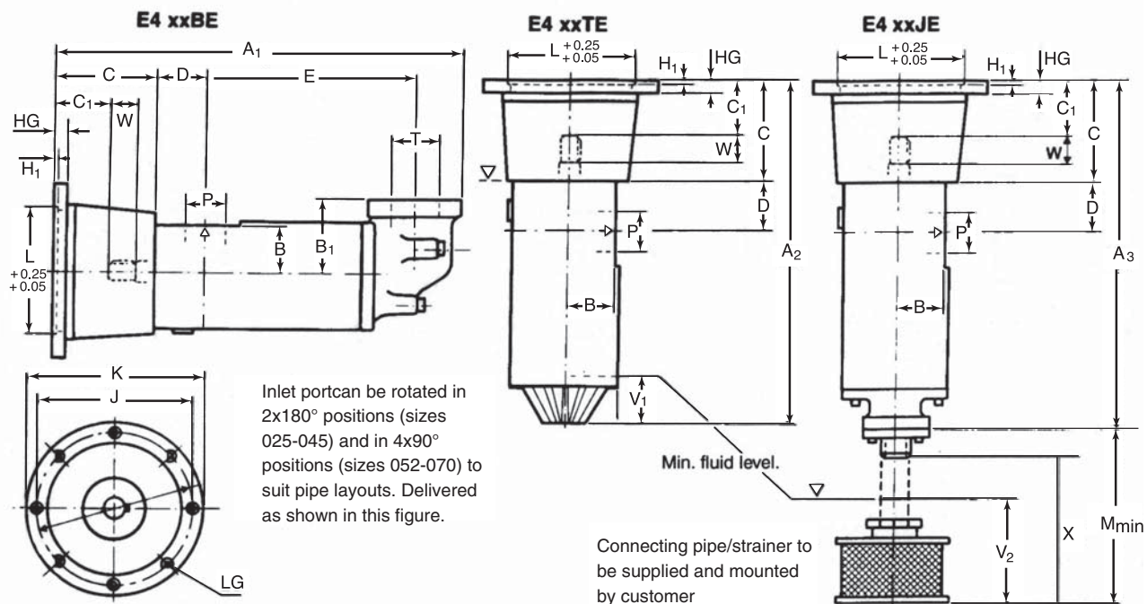
Inlet dimensions (mm)
