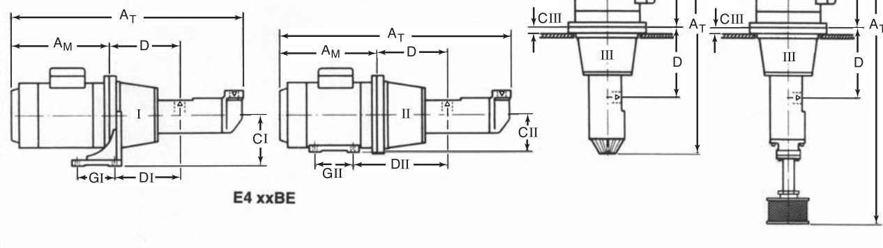
Pump Unit
