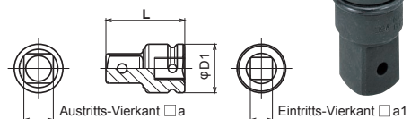
ADAPTER
