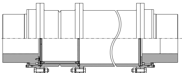
Combination Spacer Design with Shear
