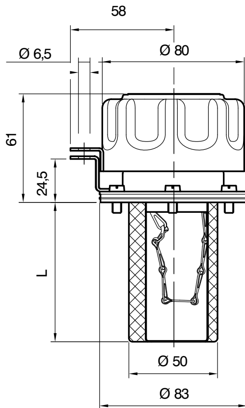
Bayonetverbindung Bayonet connection
