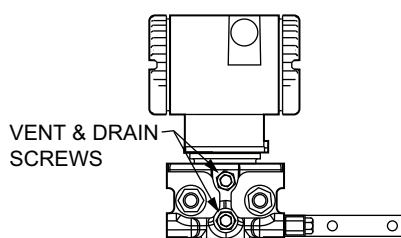
Figure 16 - Low Profile (LP2) Transmitter – Mounted to an Existing Coplanar Manifold Using Adapter Plate
