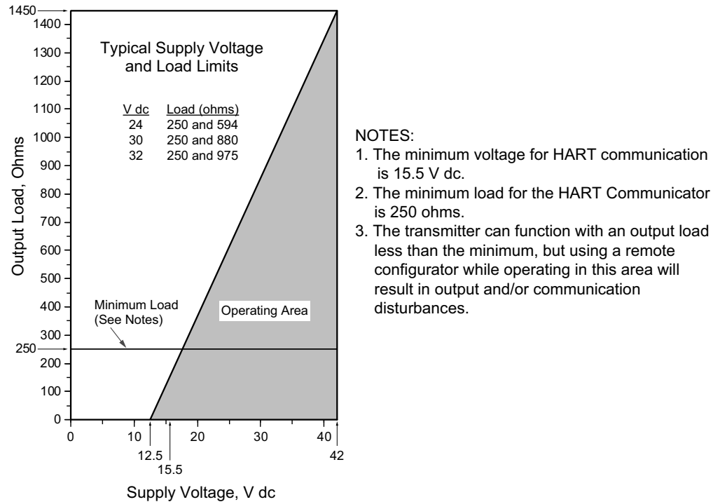
Figure 18 - 4 to 20 mA Output Supply Voltage vs Output Load
